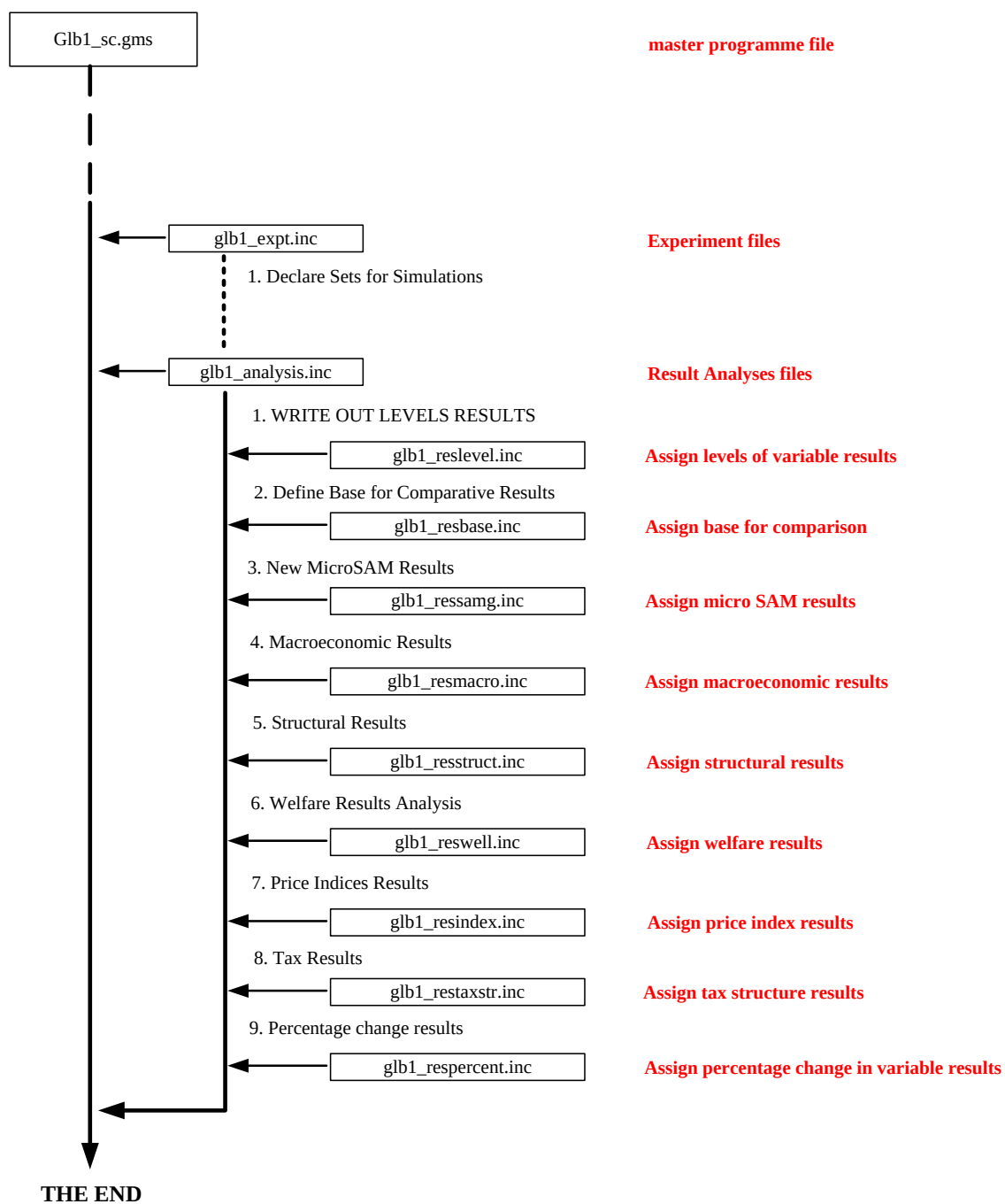
Figure 14.1 STAGE Results Analysis File Structure
